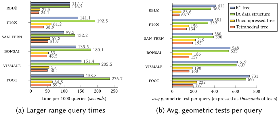
Fig. 9. Larger range query results for the R*-tree (based on the middle branching factor), the IA data structure, and the uncompressed and SRE-compressed PT-T Tetrahedral kD-trees. The IA data structure has hit ratios of 51% and 92% for RBL and F16 datasets (marked with \otimes ).
