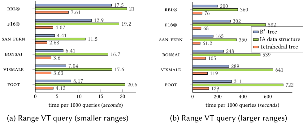
Fig. 10. Range Vertex-Tetrahedron (VT) query results for the R^* -tree (based on the middle branching factor), the IA data structure, and the SRE-compressed PT-T Tetrahedral kD-tree. The IA data structure cannot fully answer the query on some datasets (marked with \otimes ).
