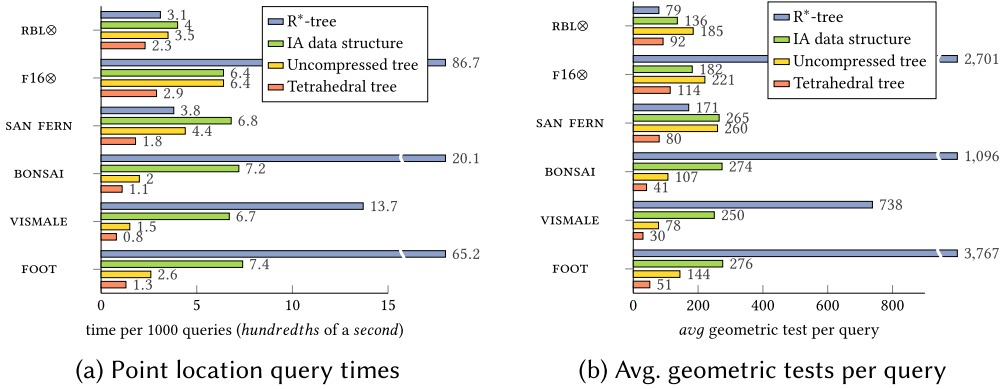
Fig. 7. Point location results for the R*-tree (based on the middle branching factor), the IA data structure, and the uncompressed and SRE-compressed PT-T Tetrahedral kD-trees. The IA data structure has hit ratios of 50% and 74% for RBL and F16 datasets (marked with ⊗), respectively.
