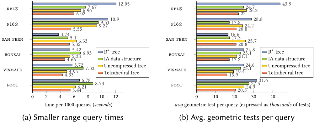
Fig. 8. Smaller range query results for the R*-tree (based on the middle branching factor), the IA data structure, and the uncompressed and SRE-compressed PT-T Tetrahedral kD-trees. The IA data structure has hit ratios of 43% and 72% for RBL and F16 datasets (marked with \otimes ), respectively.
